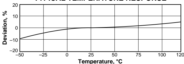
TYPICAL TEMPERATURE RESPONSE
