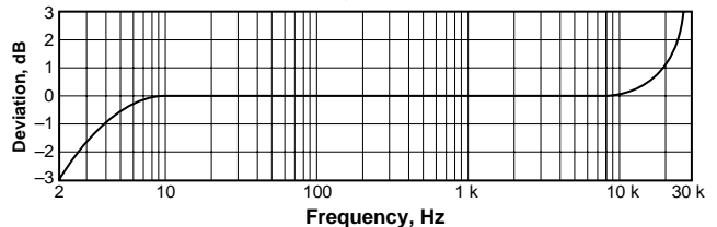
TYPICAL FREQUENCY RESPONSE
